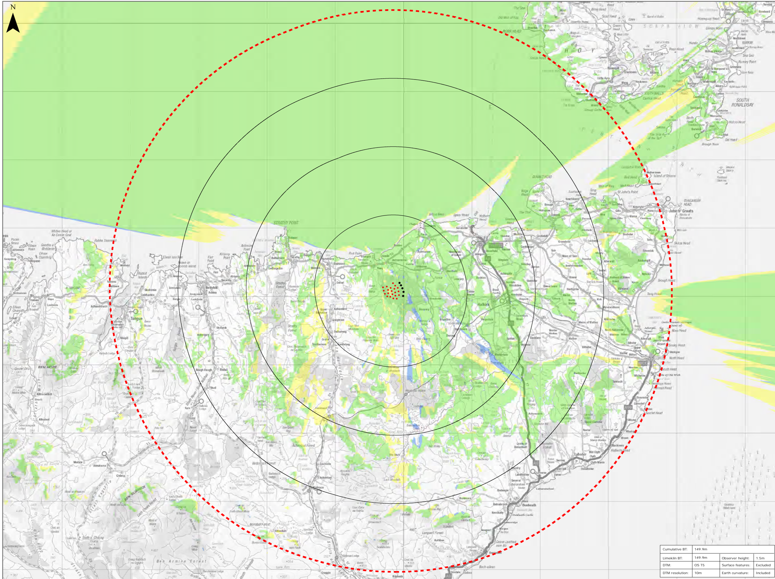
Figure 9.25: Cumulative ZTV with Limekiln Extension
