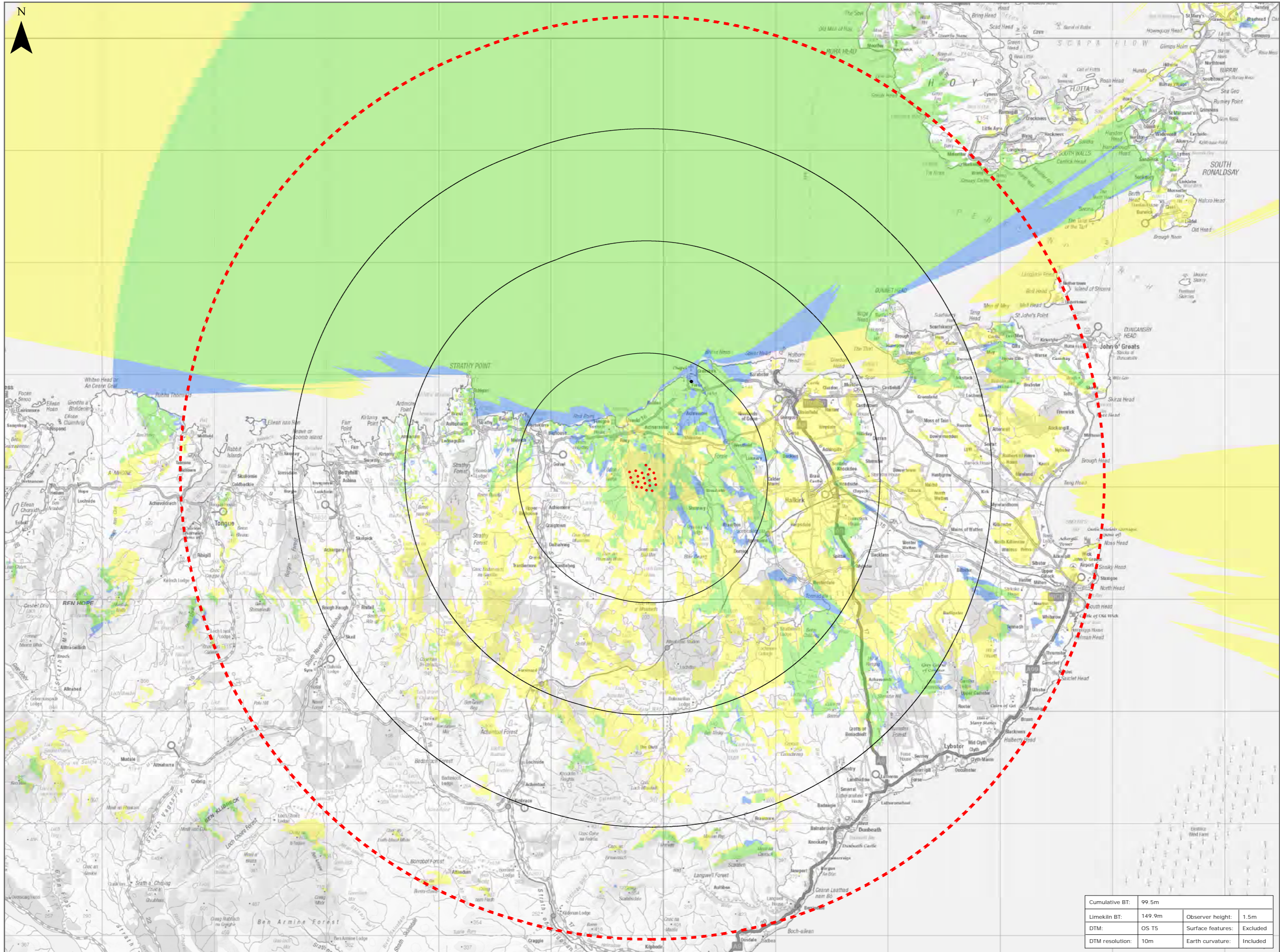
Figure 9.24: Cumulative ZTV with Hill of Lybster
