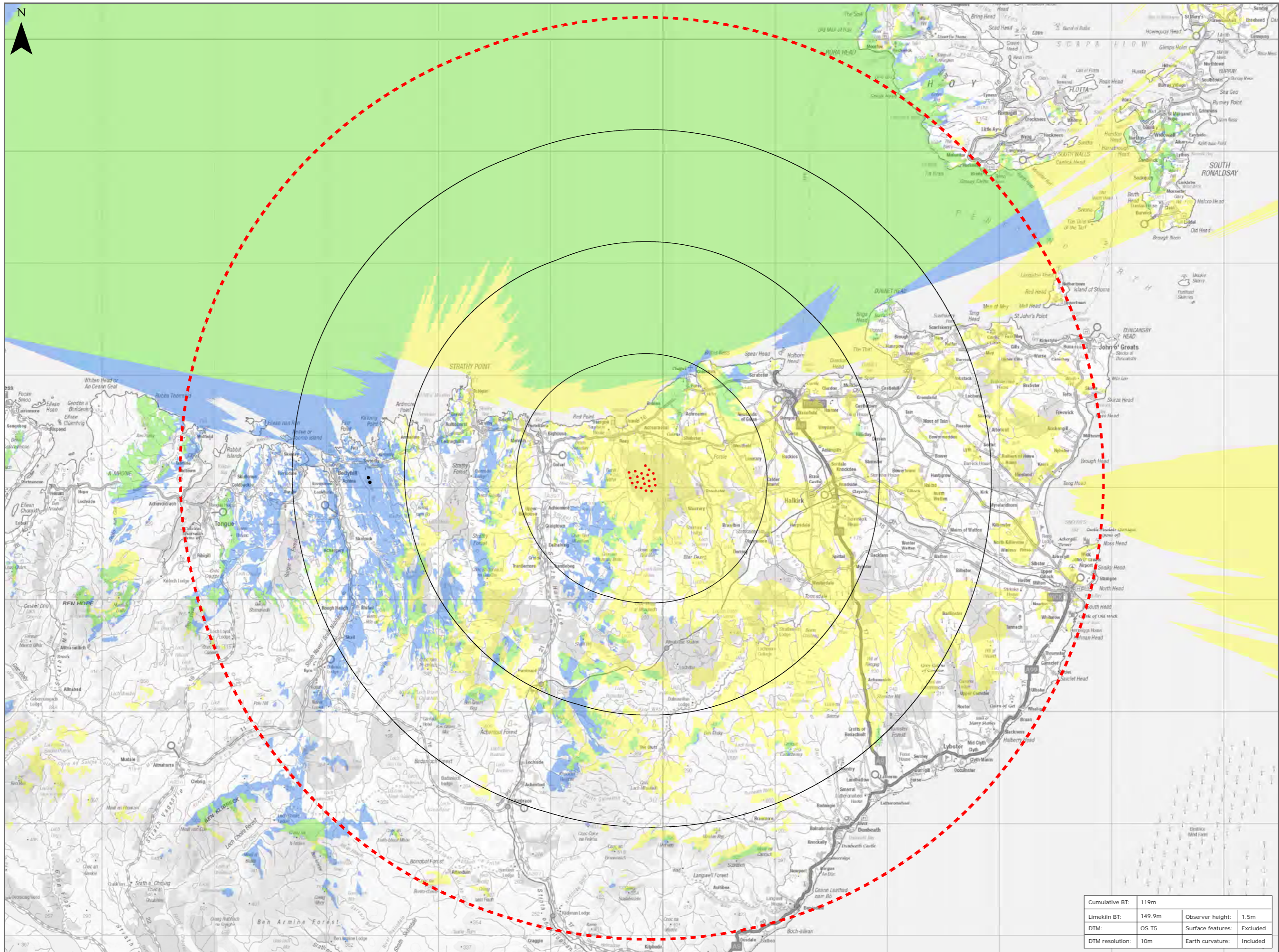
Figure 9.19: Cumulative ZTV with Bettyhill
