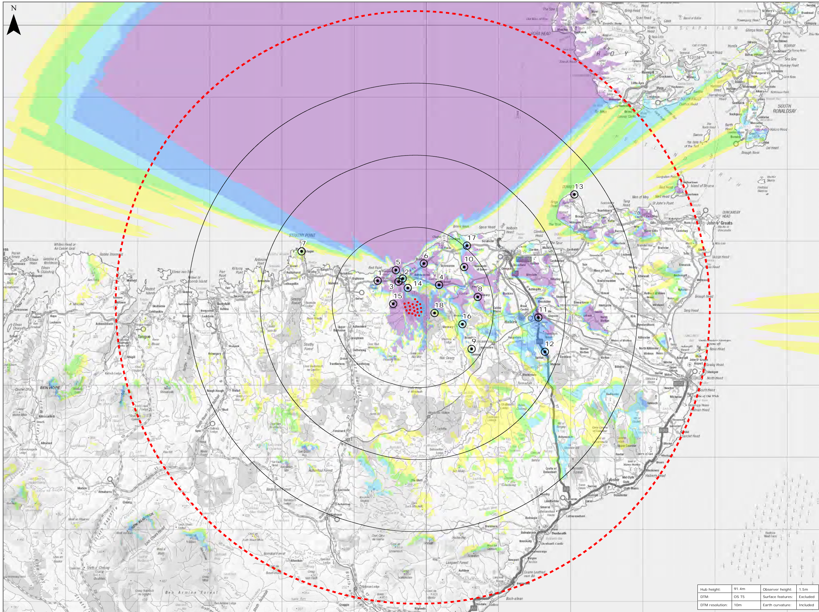
Figure 9.9a: Hub Height ZTV
