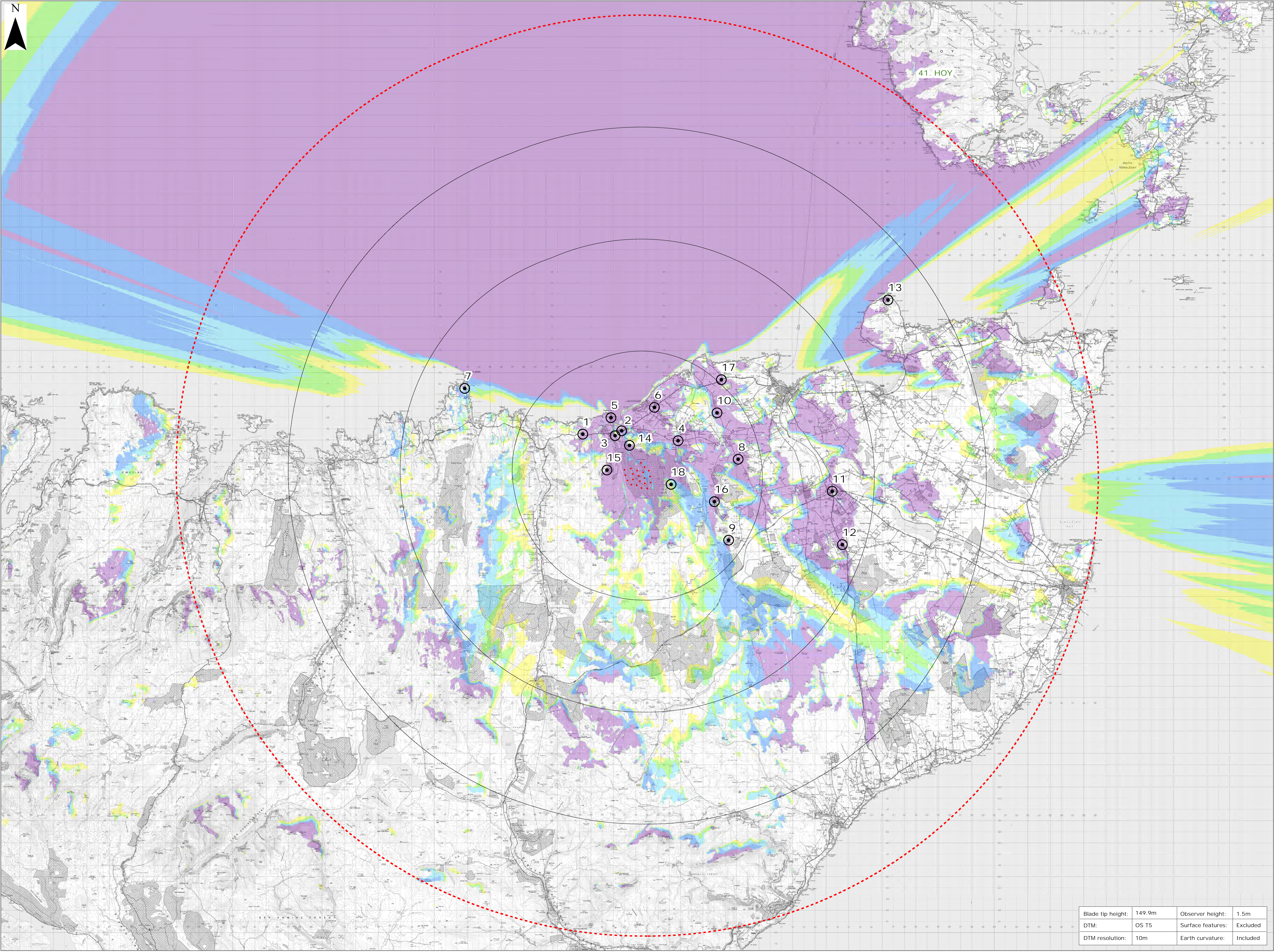
Figure 9.8b: Blade Tip ZTV with Viewpoints (A1)
