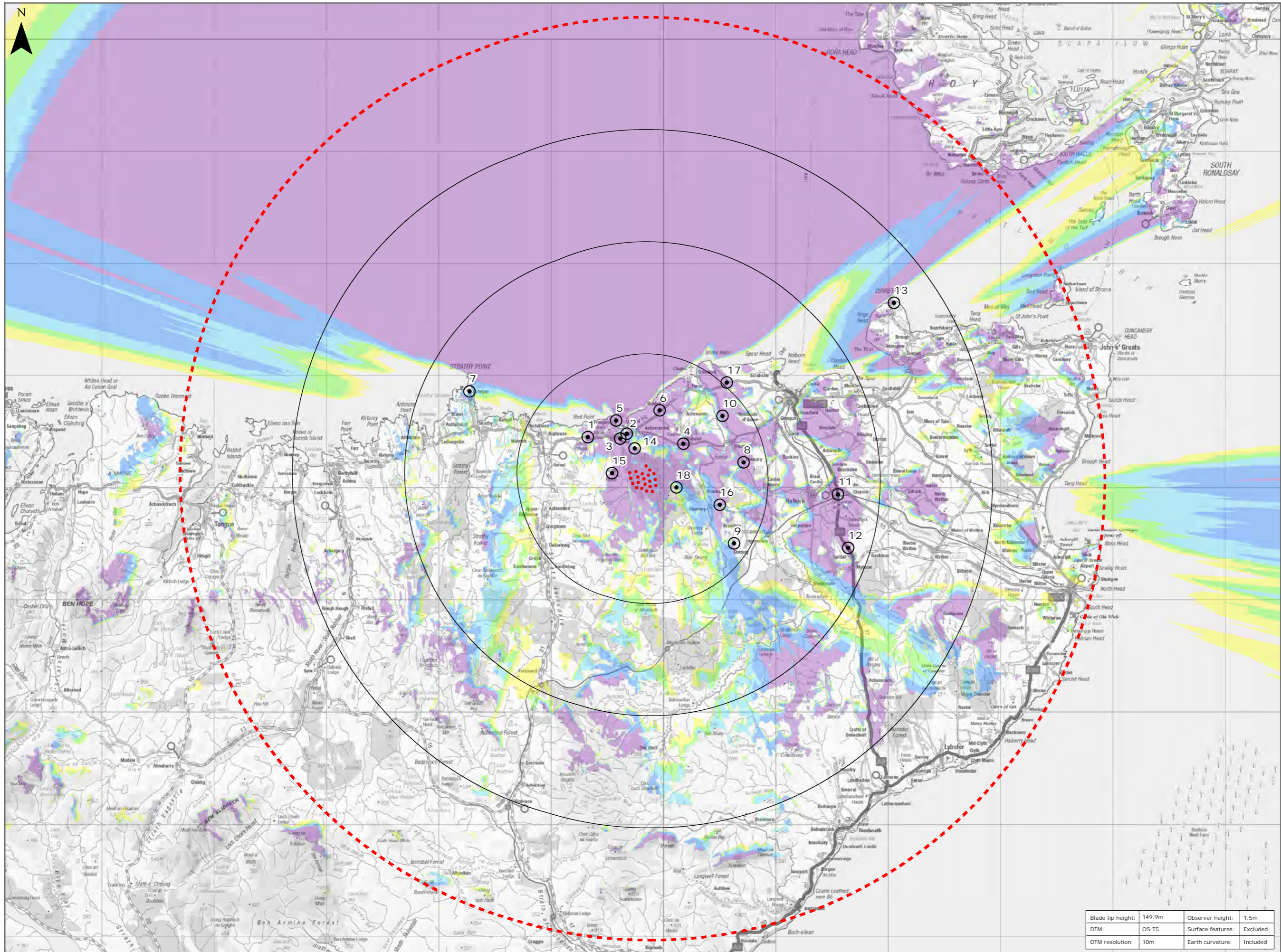
Figure 9.8a: Blade Tip ZTV
