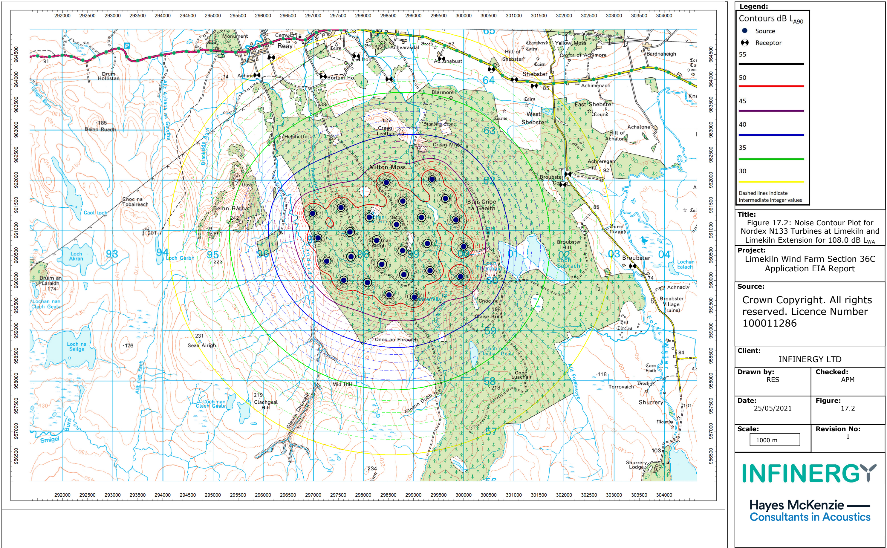
Figure 17.2: Noise Contour Plot for Nordex N133 Turbines at Limekiln and Limekiln Extension
