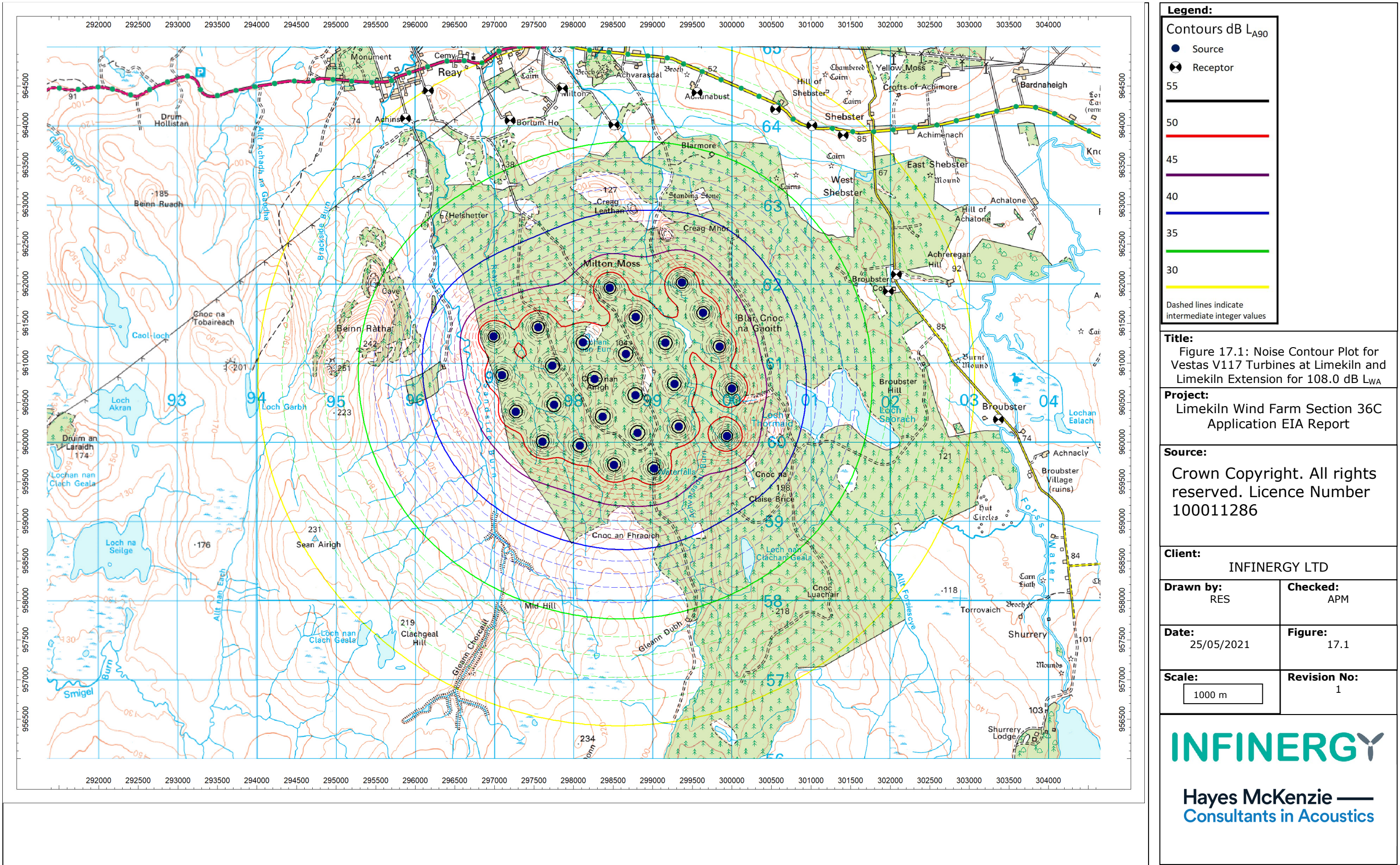
Figure 17.1: Noise Contour Plot for Vestas V117 Turbines at Limekiln and Limekiln Extension
