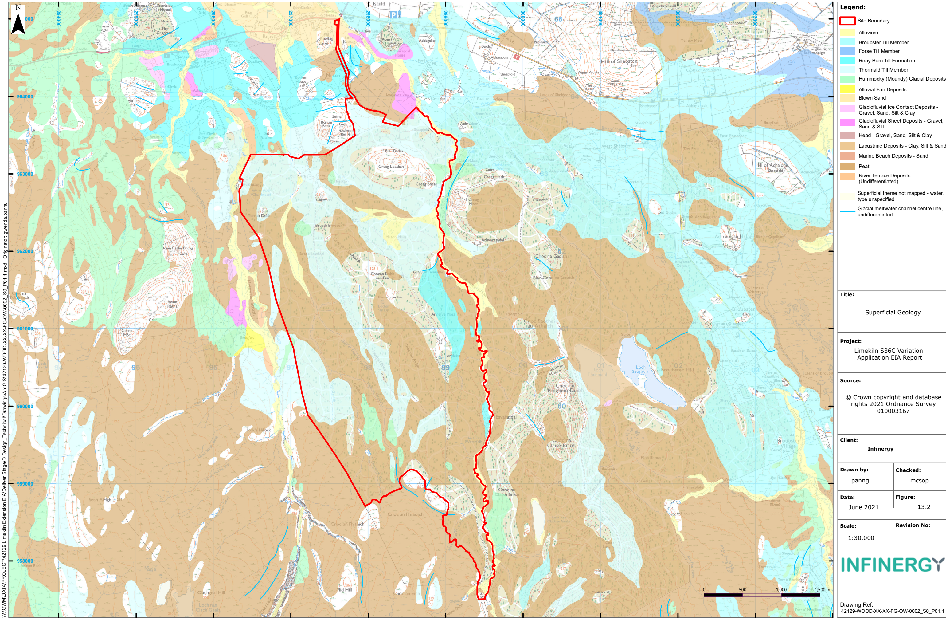
Figure 13.2: Superficial Geology
