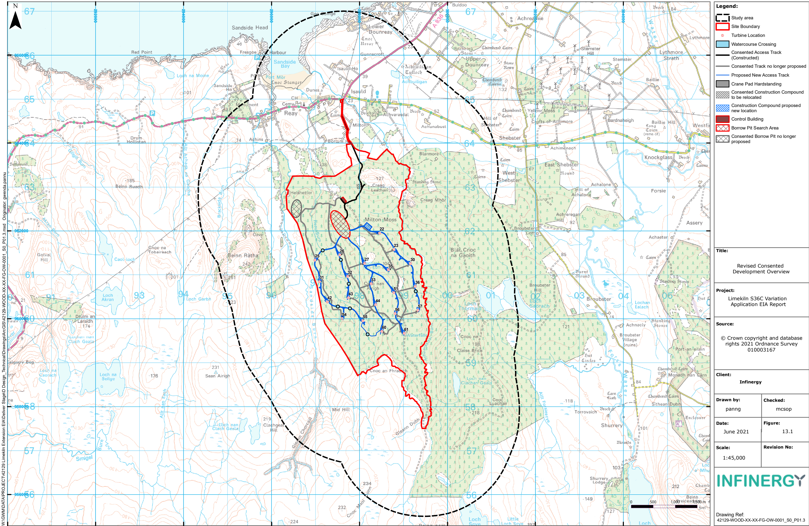
Figure 13.1: Revised Consented Development Overview
