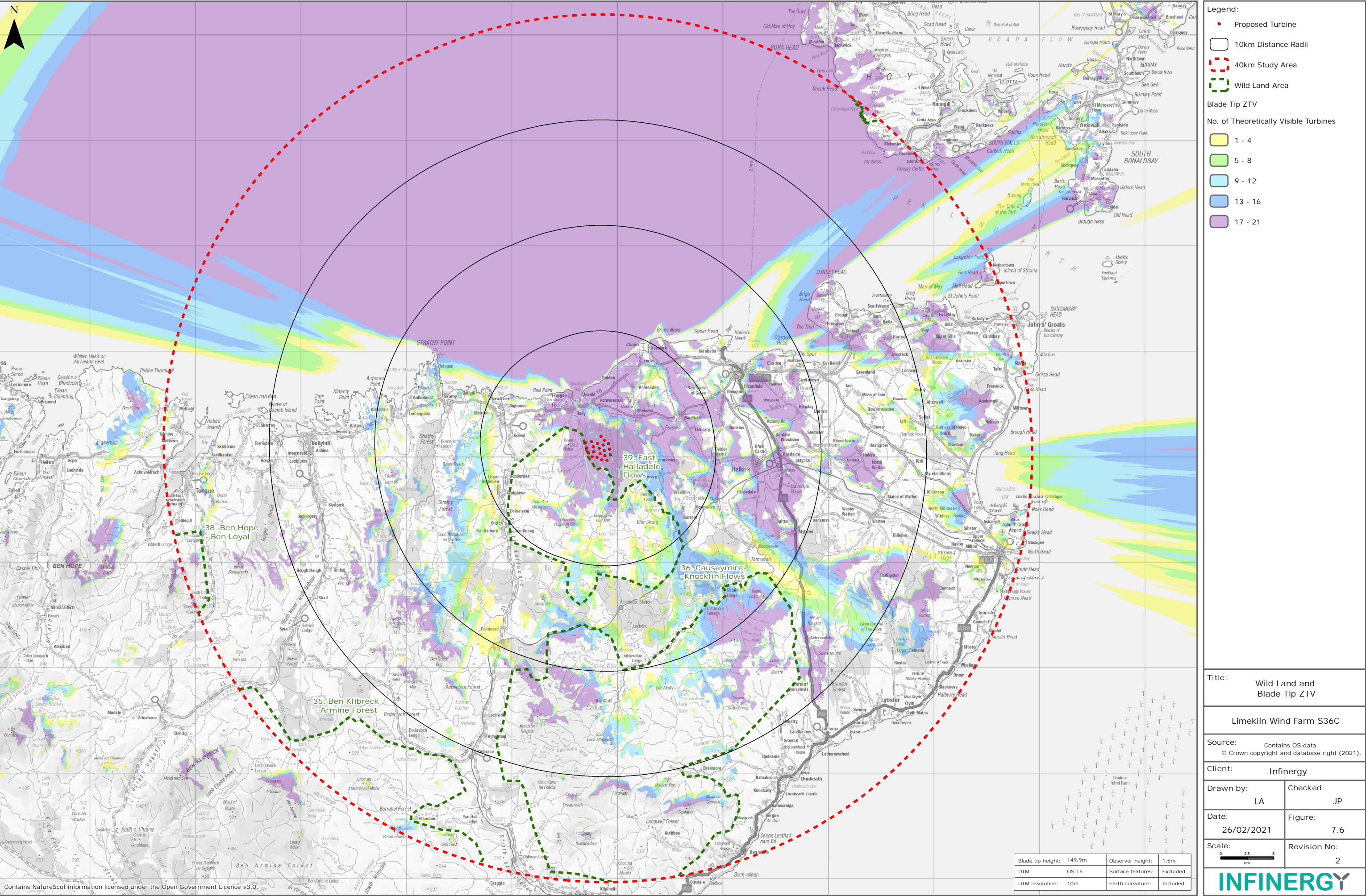
Figure 7.6: Wild Land and Blade Tip ZTV
